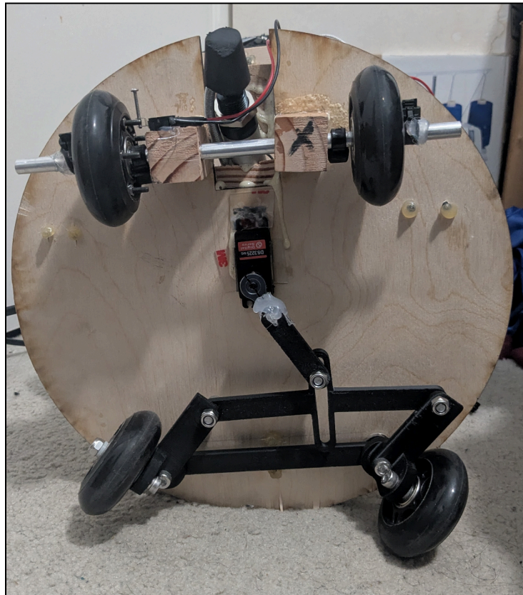
Figure 4: Bottom view of the physical robot, showcasing steering mechanism and rear axle.
