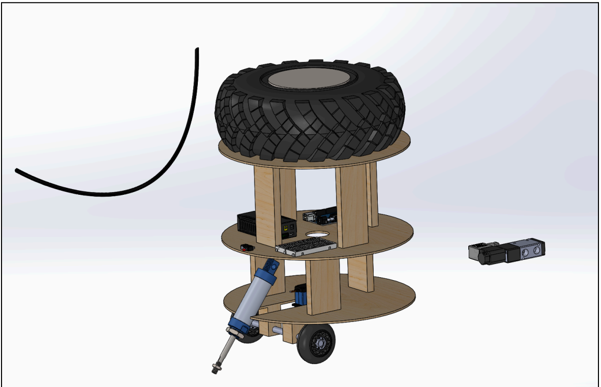
Figure 2: CAD Isometric view of wooden structure of the robot.
