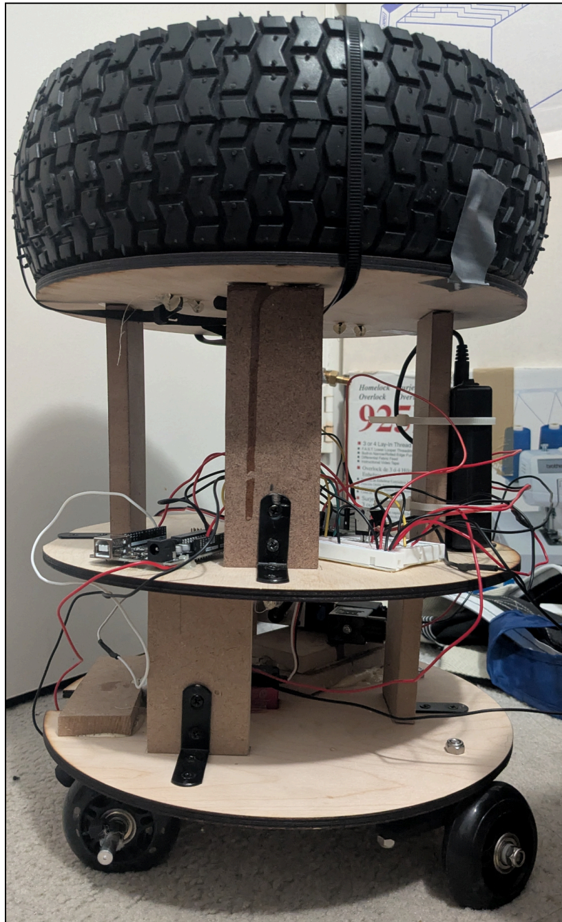
Figure 5: Right view of physical robot, showcasing the electrical components being mounted.
