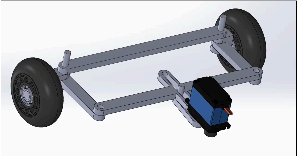
Figure 1: CAD Steering mechanism.
